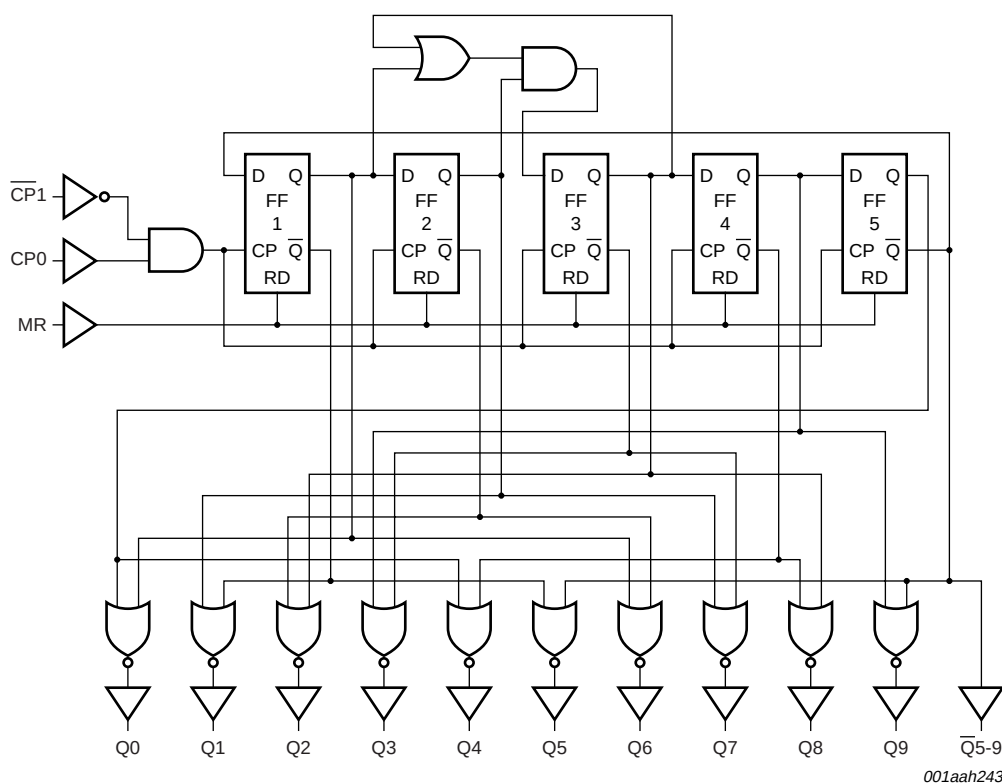
Fig 2. Logic diagram
