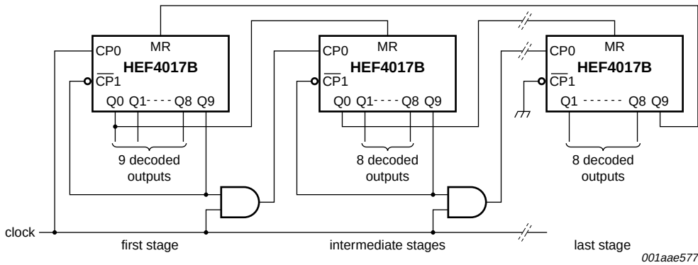
Fig 11. Counter expansion
