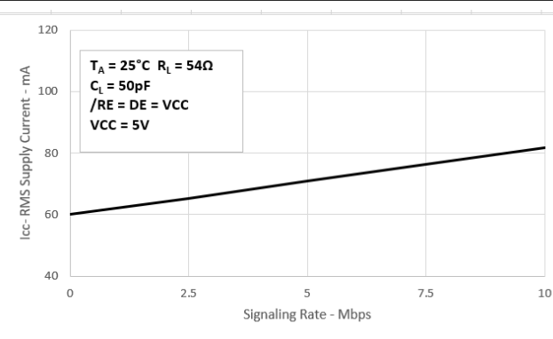
Figure 6-4. RMS Supply Current vs Signaling Rate
