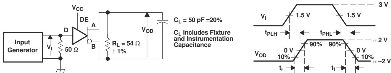
Figure 7-2. Test Circuit and Definitions for the Driver Common-Mode Output Voltage
