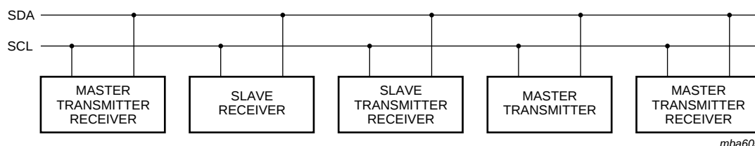
Fig 15. System configuration
