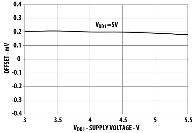
Figure 4: Input Offset vs. Supply Voltage V_{DD2}
