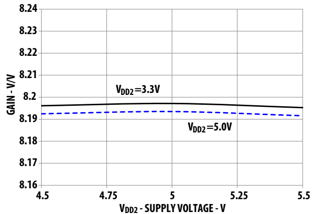
Figure 6: Gain vs. Supply Voltage V_{DD1}
