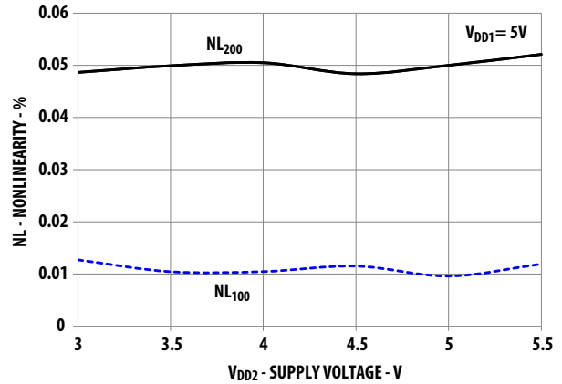
Figure 10: Nonlinearity vs. Supply Voltage V_{DD2}
