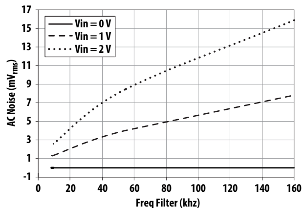
Figure 12: AC Noise vs. Filter Freq vs. Vin
