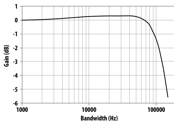
Figure 14: Frequency Response
