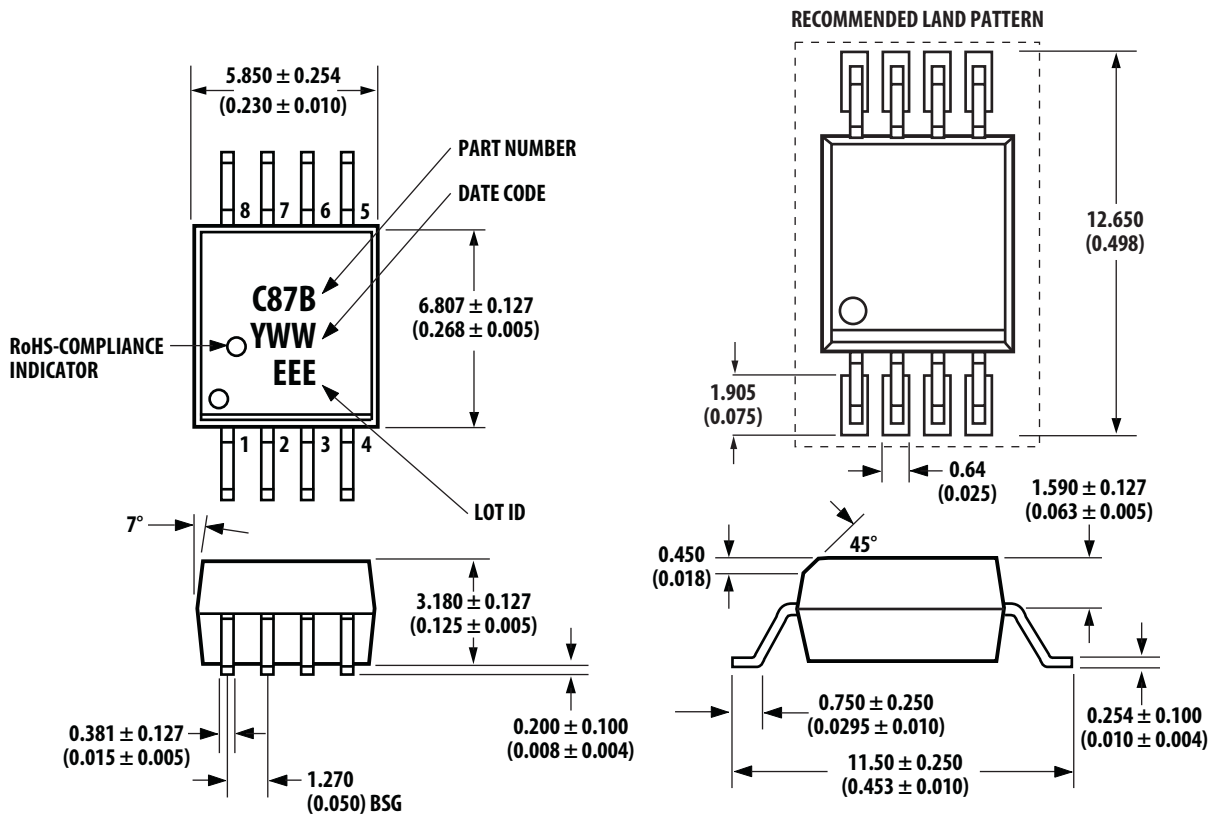
Figure 2: SSO-8 Package
