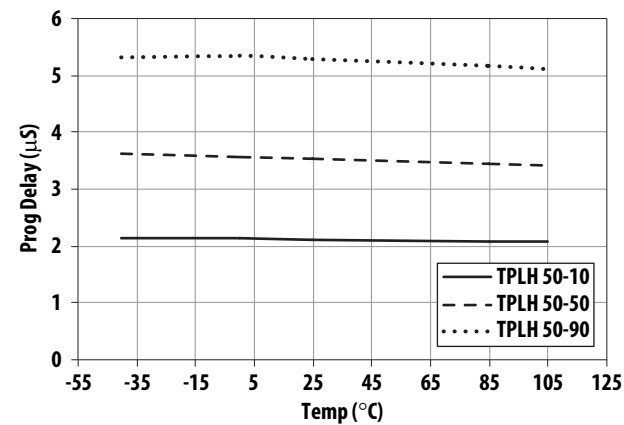
Figure 16: Propagation Delay vs Temperature
