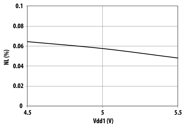
Figure 9: Non-Linearity vs. Supply VDD1
