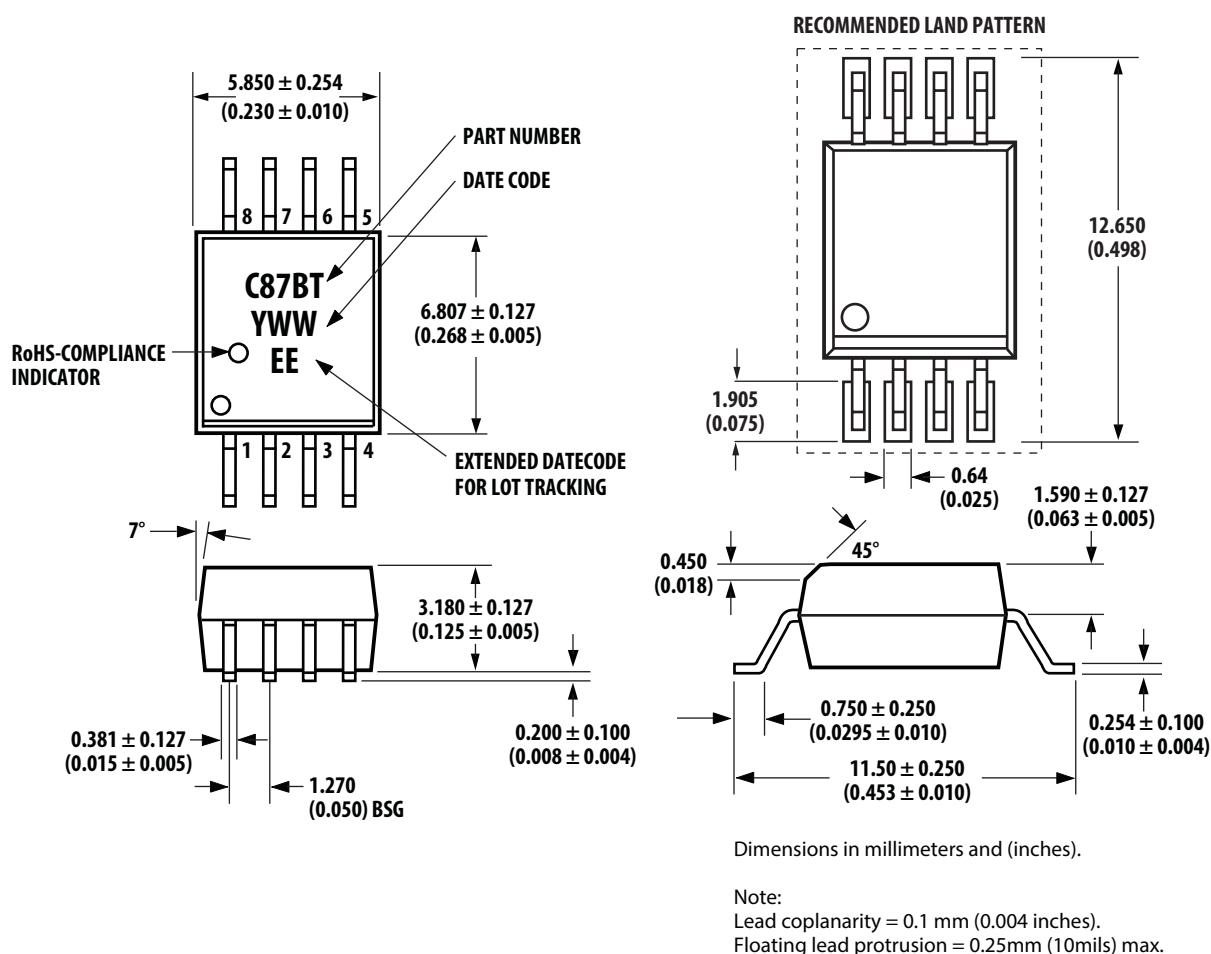
Figure 5: Package Outline Drawing
