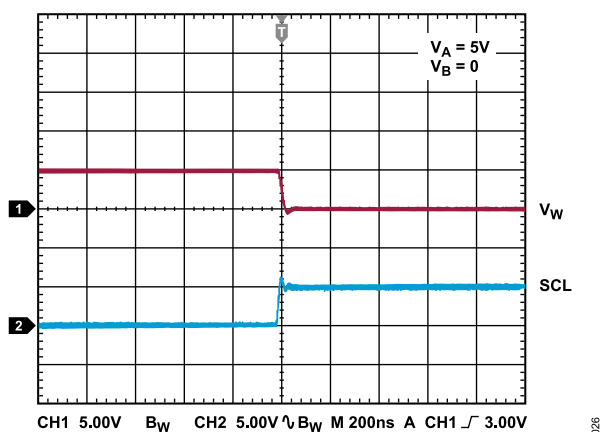
Figure 27. Midscale Glitch, Code Transition from 0x80 to 0x7F
