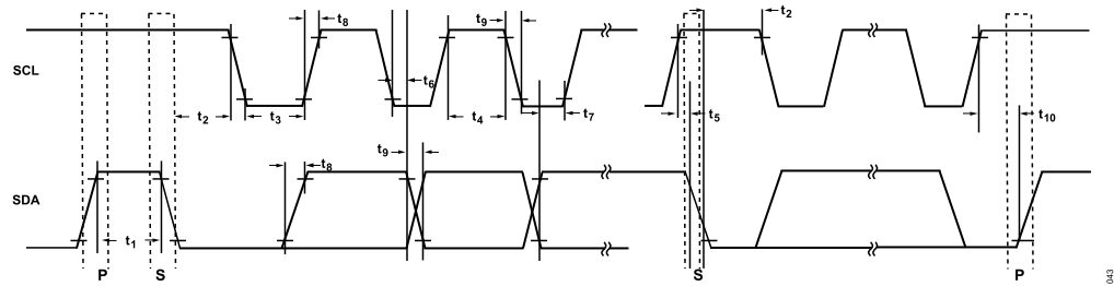
Figure 2. I 2 C Interface Detailed Timing Diagram
