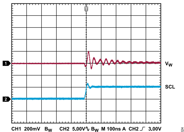
Figure 25. Large Signal Settling Time, Code 0xFF \geq 0x00
