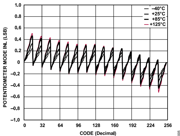
Figure 6. INL vs. Code vs. Temperature, V_{DD} = 5\text{ V}
