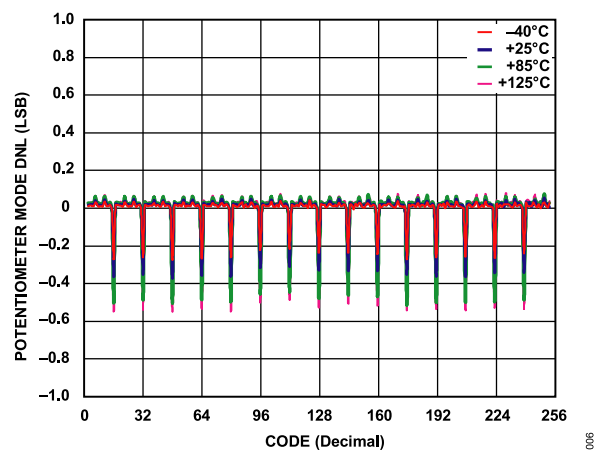
Figure 7. DNL vs. Code vs. Temperature, V_{DD} = 5\text{ V}
