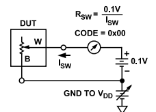
Figure 33. Test Circuit for Incremental On Resistance
