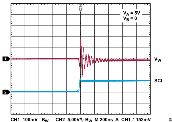
Figure 26. Digital Feedthrough
