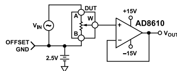
Figure 32. Test Circuit for Gain vs. Frequency
