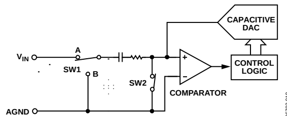
Figure 16. ADC Acquisition Phase
