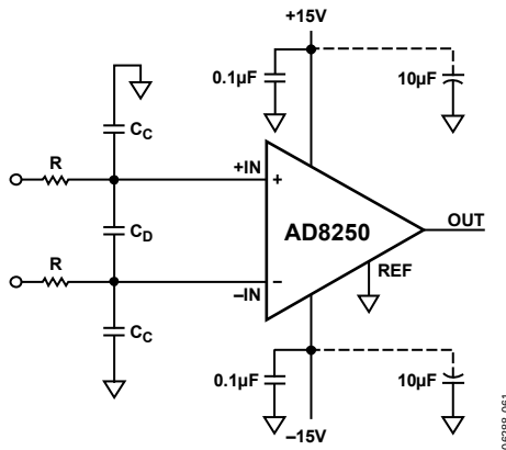
Figure 54. RFI Suppression
