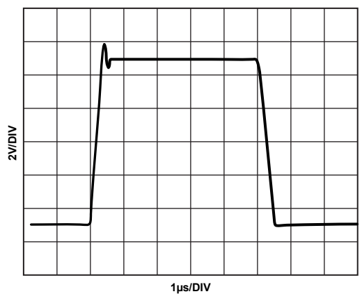
Figure 27. Large-Signal Pulse Response, Gain = \frac{1}{2}
