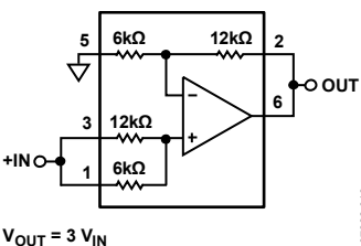
Figure 47. Noninverting Amplifier, G = 3
