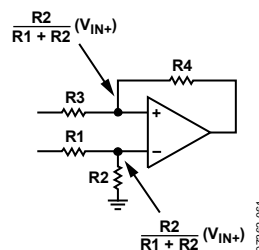
Figure 39. Voltage Division in the Difference Amplifier Configuration
