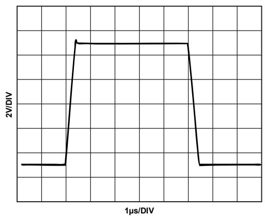
Figure 28. Large-Signal Pulse Response, Gain = 2
