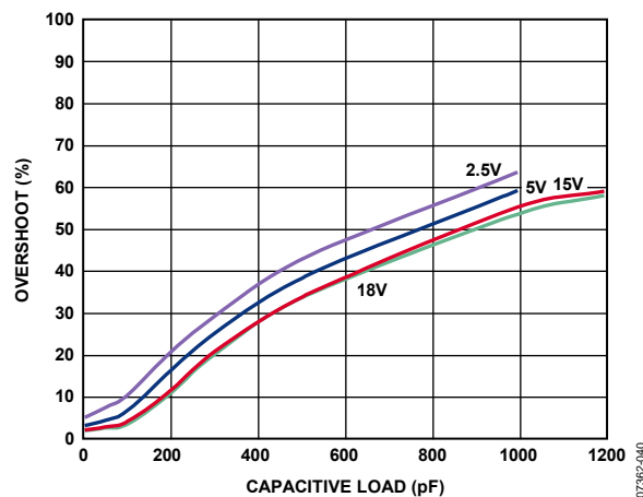
Figure 26. Small-Signal Overshoot vs. Capacitive Load, Gain = 2, 600 \Omega in Parallel with Capacitive Load
