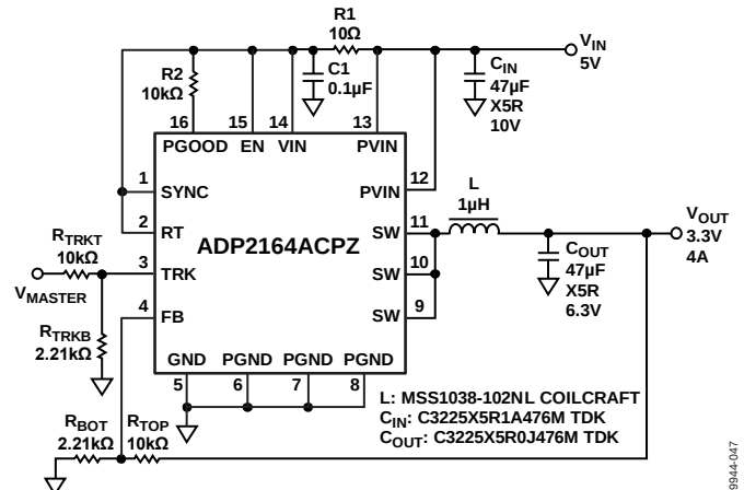
Figure 47. 3.3 V, 4 A, 1.2 MHz Step-Down Regulator, Tracking Mode
