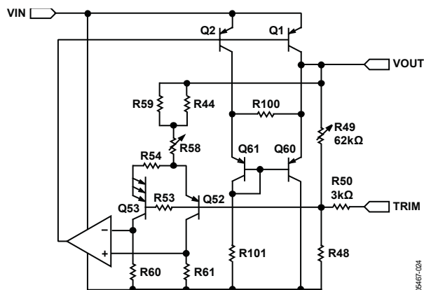
Figure 36. Simplified Schematic
