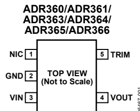
Figure 1. 5-Lead TSOT (UJ-5)
