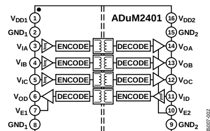
Figure 2. ADuM2401
