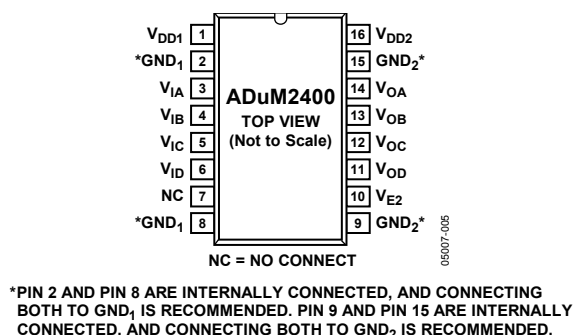
Figure 5. ADuM2400 Pin Configuration
