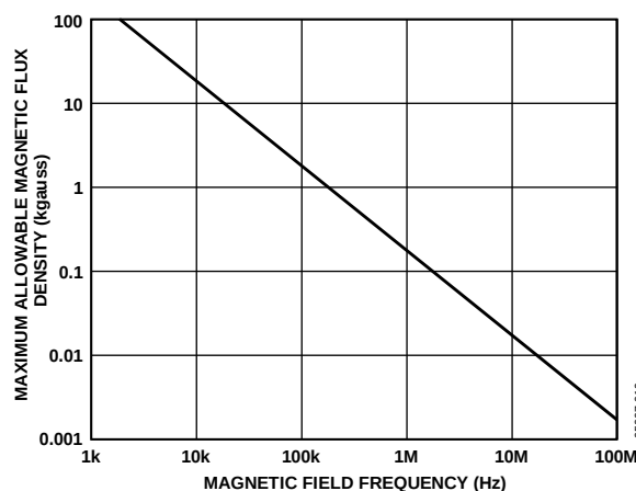
Figure 19. Maximum Allowable External Magnetic Flux Density
