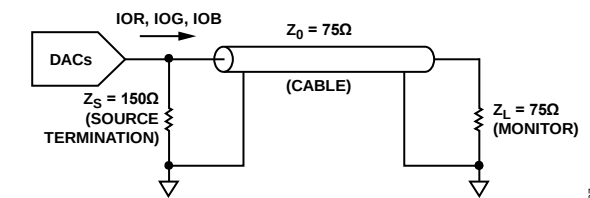
Figure 8. Analog Output Termination for RS-343A
