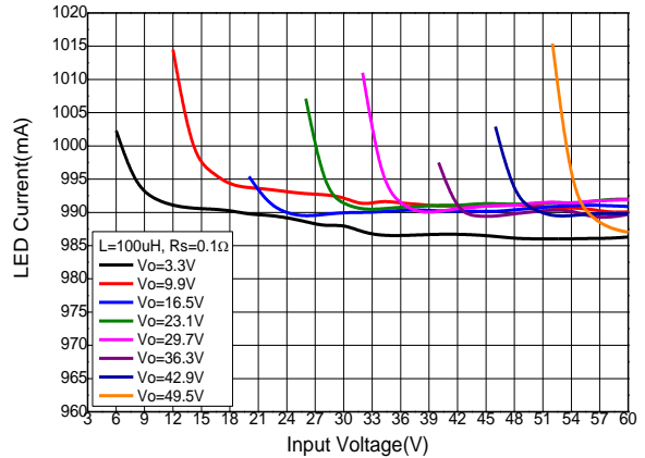
LED Current vs. Input Voltage ( R_s=0.1\Omega , L=100\mu\text{H} )
