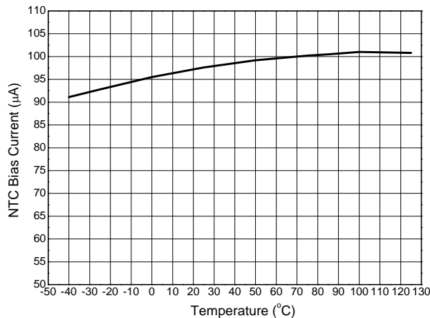
NTC Bias Current vs. Temperature
