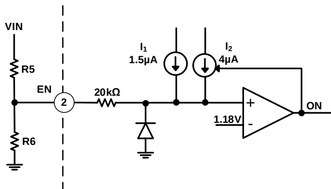
Figure 22. Programming UVLO
