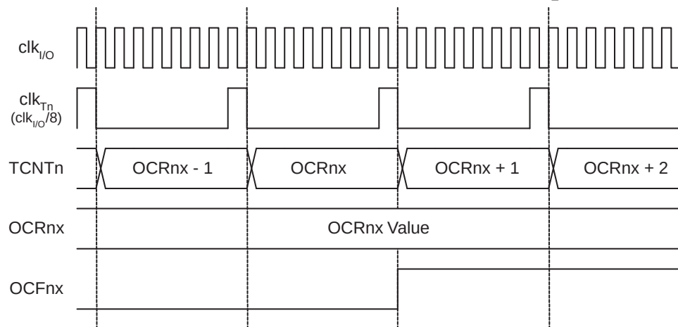
Figure 13-11. Timer/Counter Timing Diagram, Setting of OCFnx, with Prescaler ( f_{\text{clk}_{\text{I/O}}/8} )
