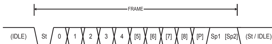
Figure 16-4. Frame Formats
