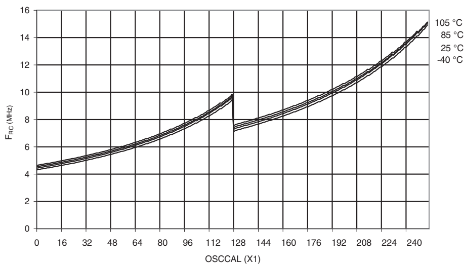
Figure 28-73. ATmega324P: Calibrated 8 MHz RC Oscillator vs. OSCAL Value
