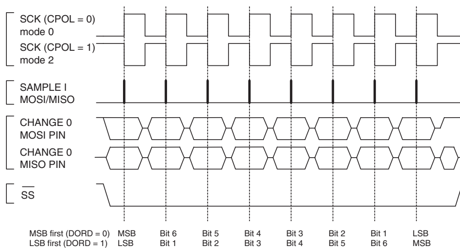
Figure 17-3. SPI Transfer Format with CPHA = 0
