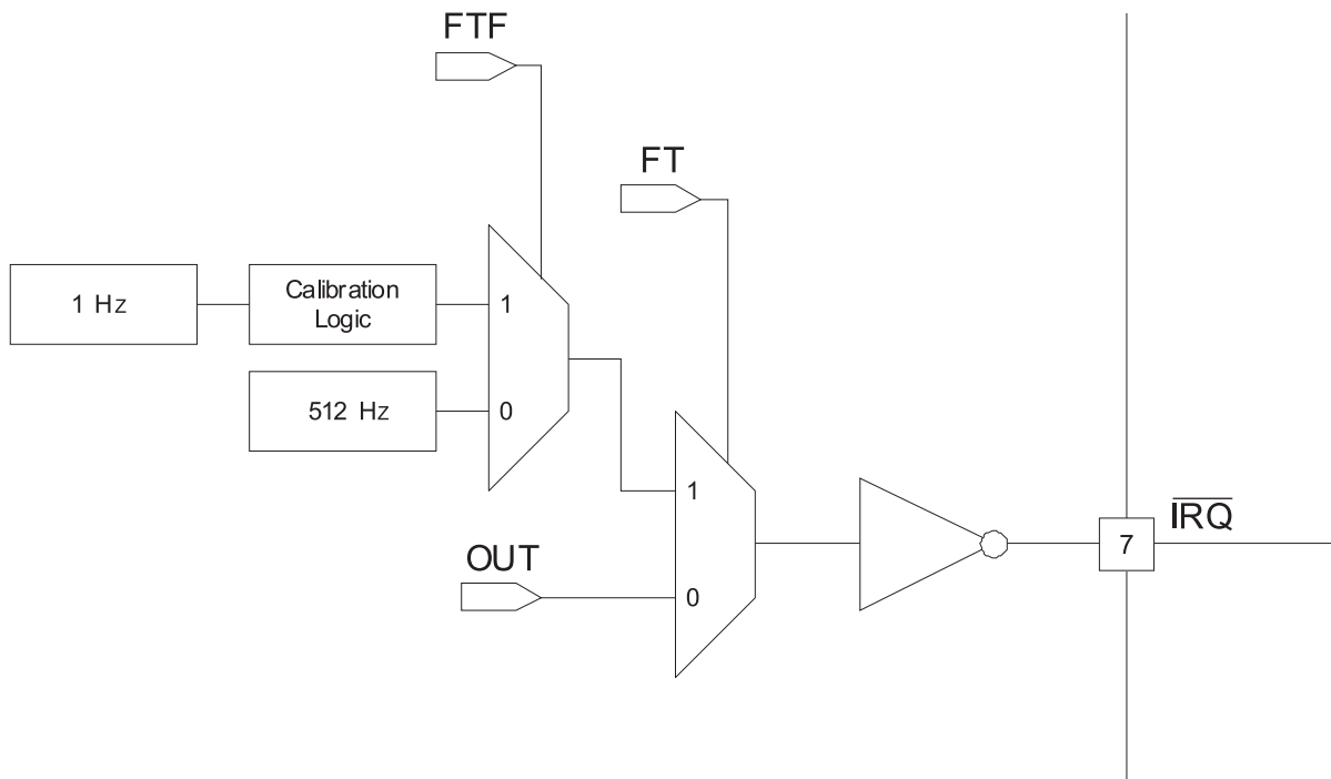
Figure 4. \overline{\text{I2C}} Pin Functional Diagram
