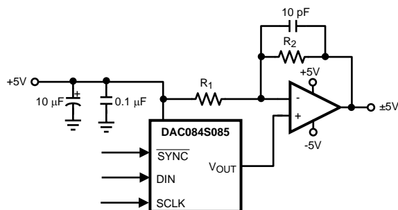
Figure 35. Bipolar Operation
