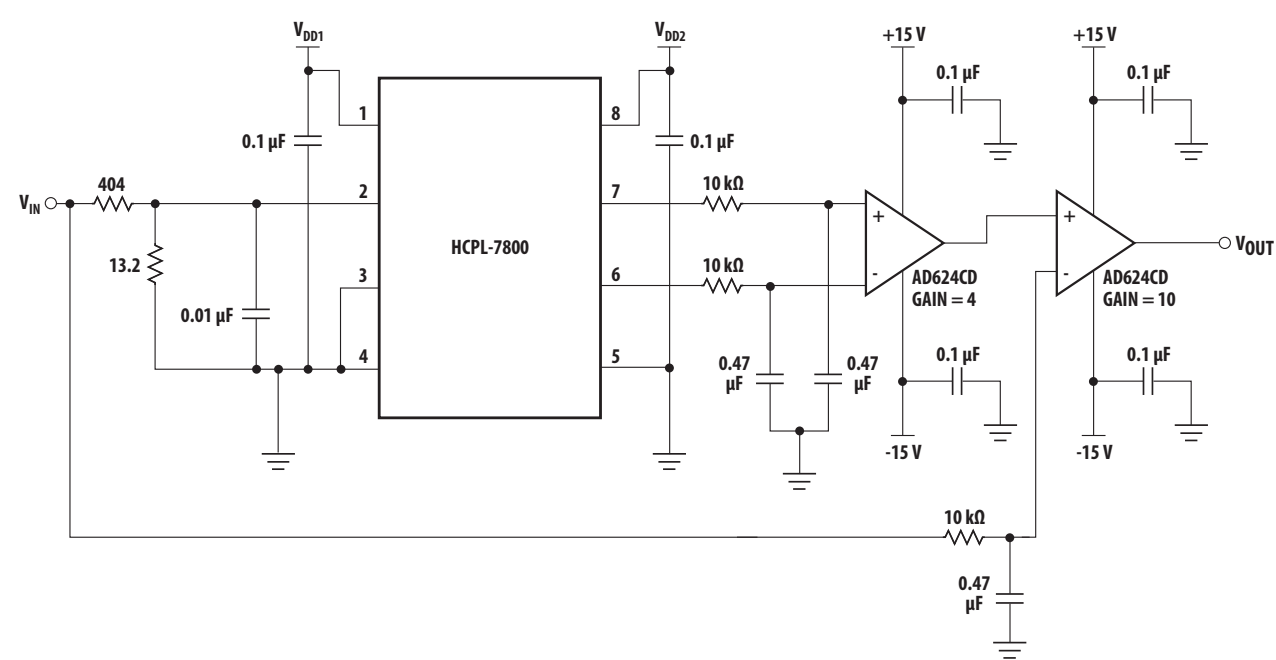
Figure 6: Gain and Nonlinearity Test Circuit
