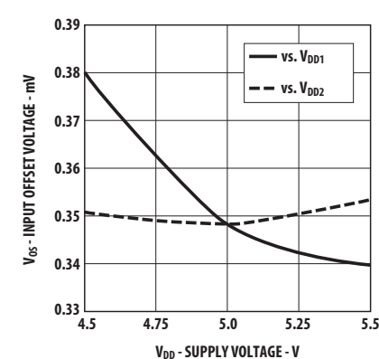
Figure 4: Input Offset vs. Supply
