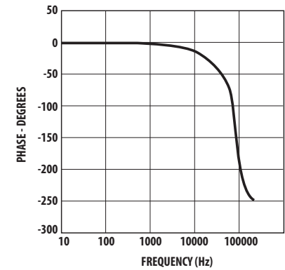
Figure 14: Phase vs. Frequency
