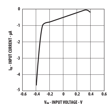
Figure 12: Input Current vs. Input Voltage
