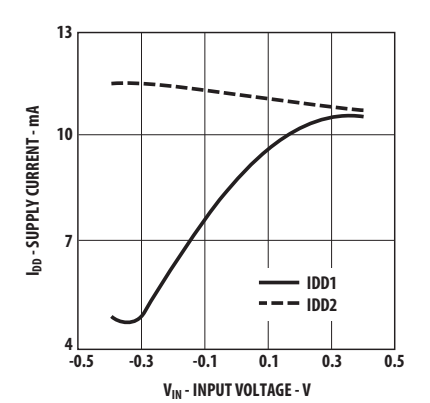
Figure 11: Supply Current vs. Input Voltage
