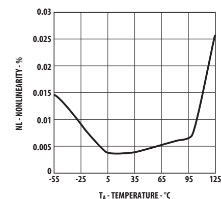
Figure 8: Nonlinearity vs. Temperature
