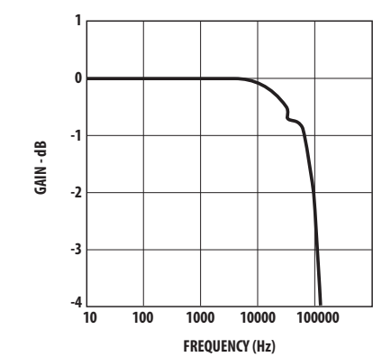
Figure 13: Gain vs. Frequency
