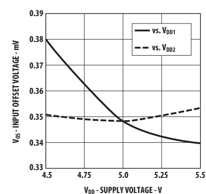
Figure 4: Input Offset vs. Supply
