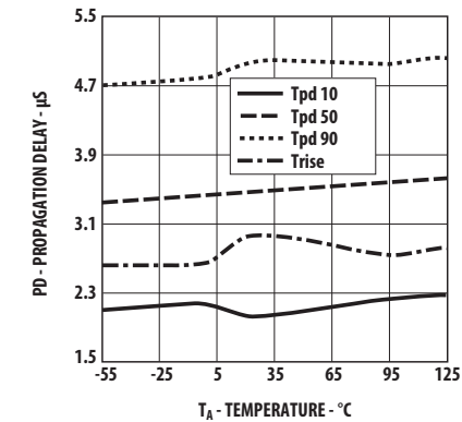
Figure 15: Propagation Delay vs. Temperature
