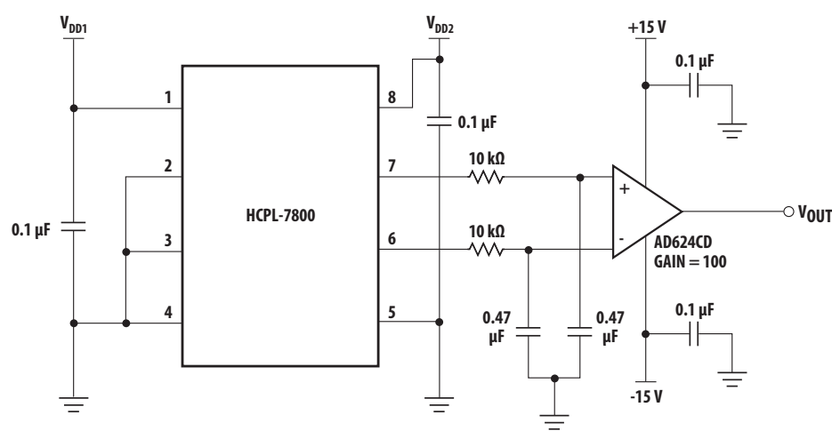
Figure 2: Input Offset Voltage Test Circuit
