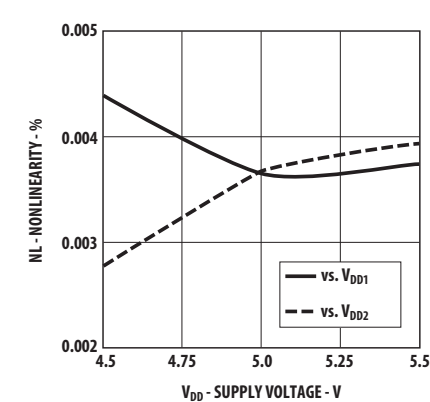
Figure 9: Nonlinearity vs. Supply
