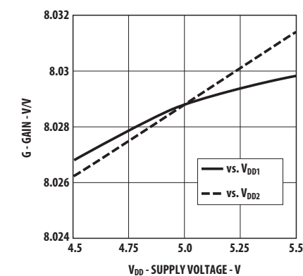
Figure 7: Gain vs. Supply
