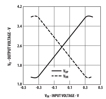
Figure 10: Output Voltage vs. Input Voltage
