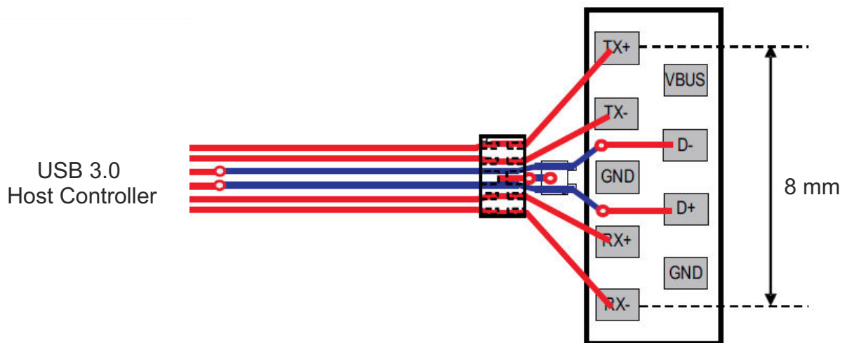
Figure 9-9. Flow-Through Routing
