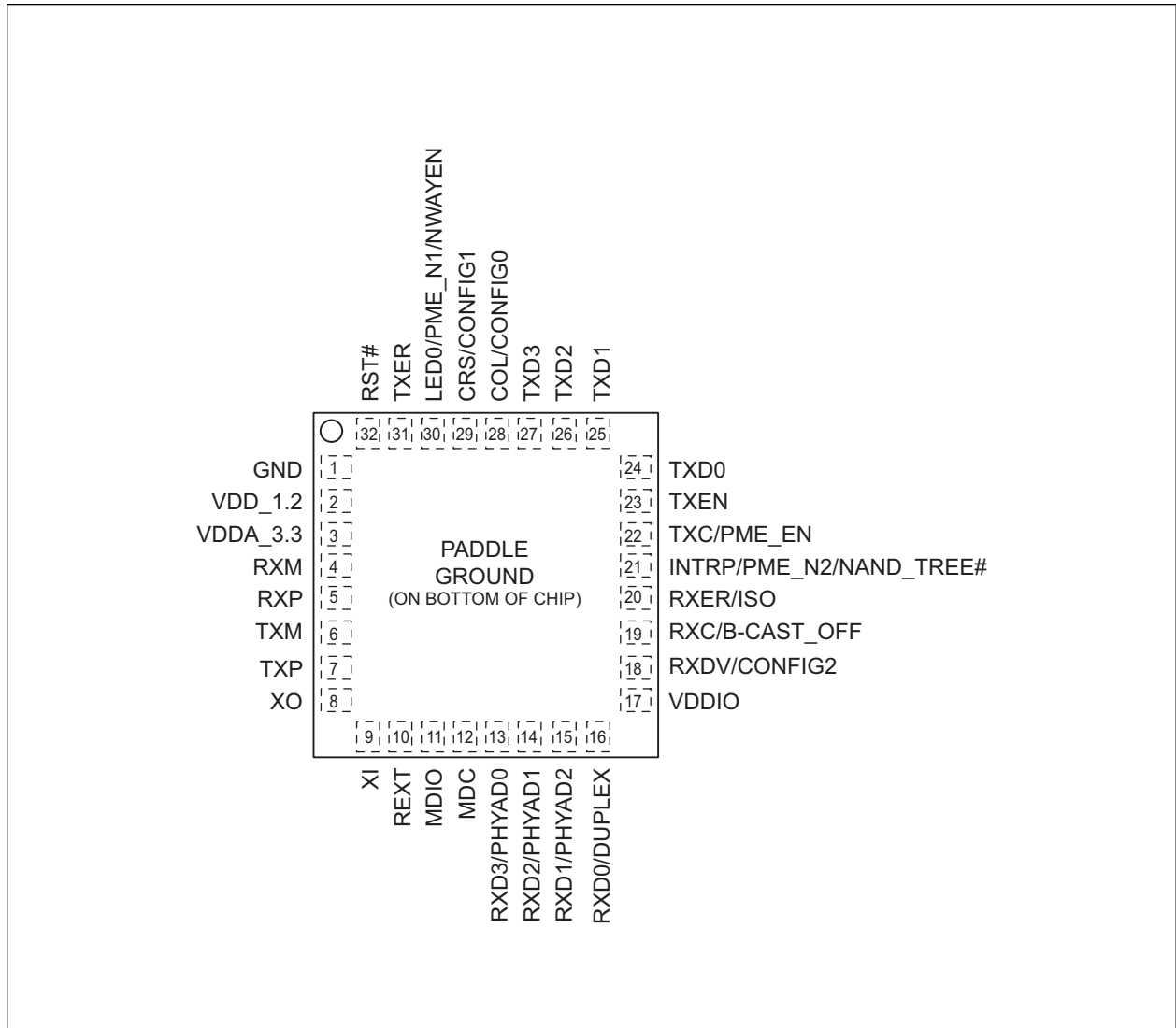
FIGURE 2-1: 32-PIN 5 MM X 5 MM VQFN ASSIGNMENT, KSZ8091MNX (TOP VIEW)
