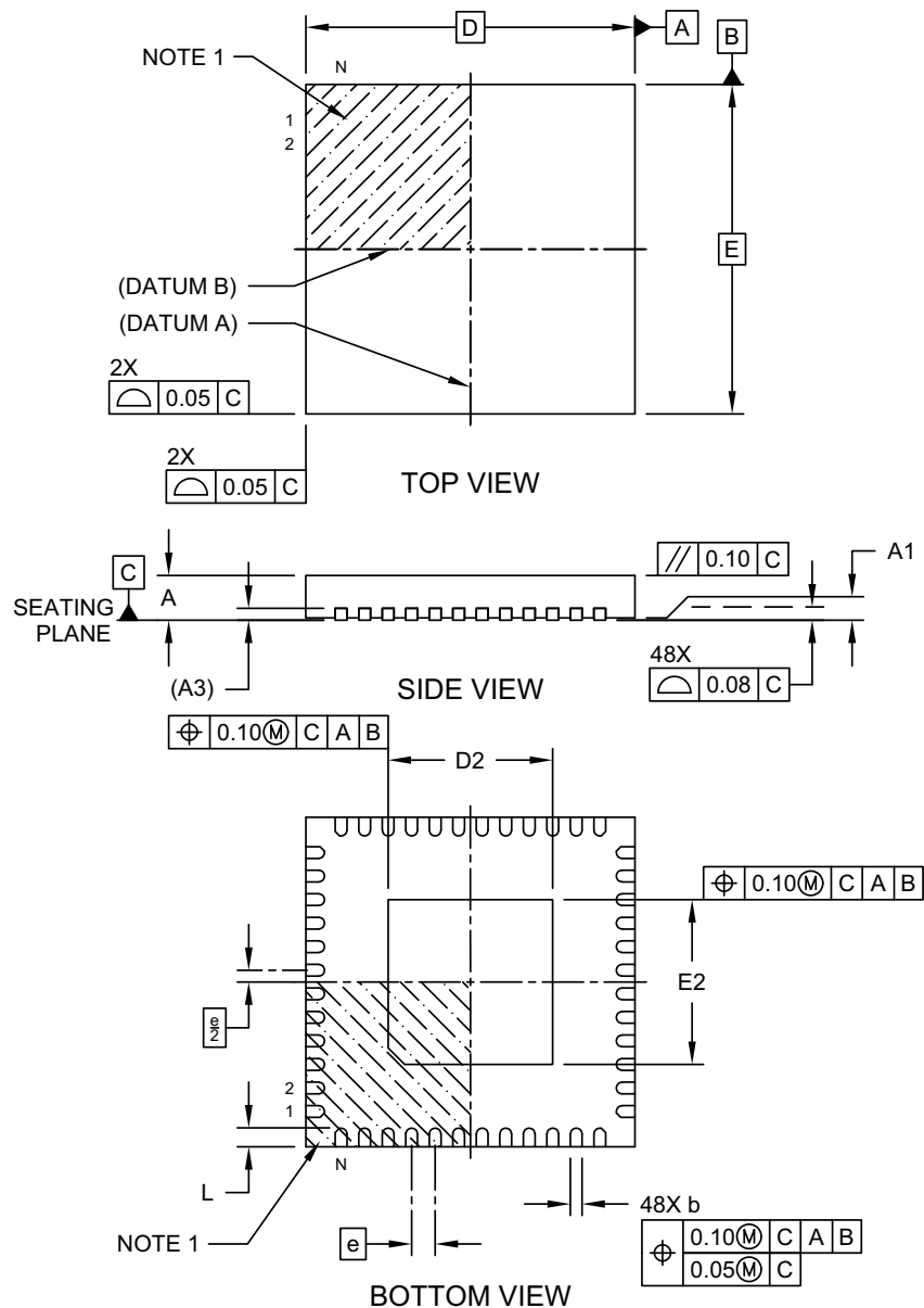
FIGURE 13-1: 48-LEAD VERY THIN PLASTIC QUAD FLAT, NO LEAD PACKAGE (PVA) - 7 MM X 7 MM X 0.9 MM BODY [VQFN] WITH 3.5 MM X 3.5 MM EXPOSED PAD; MICREL LEGACY PACKAGE MLF77Q-48L (DRAWING)
