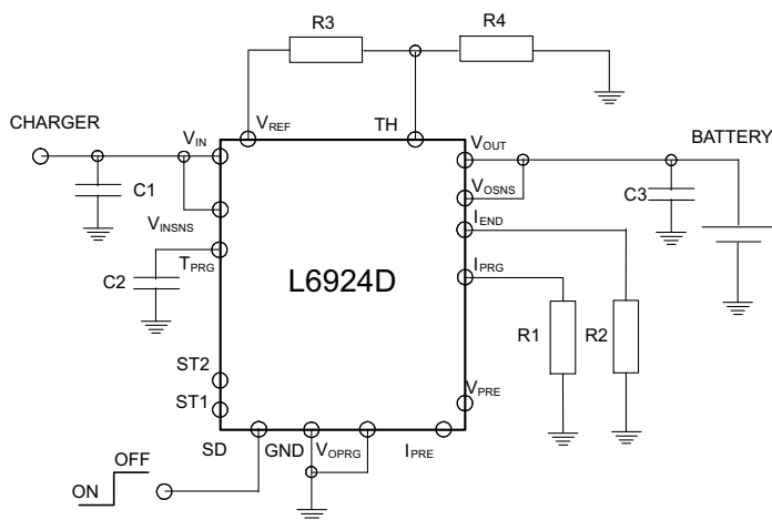
Figure 2. Basic application schematic
