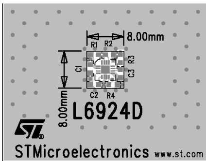
Figure 1. Minimum application size
