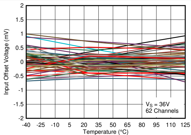
Figure 7-10. Input Offset Voltage vs. Temperature at 36
