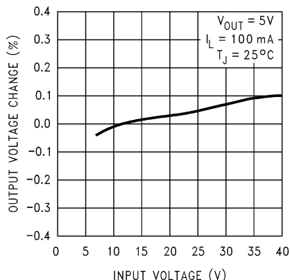
Figure 7-2. Line Regulation
