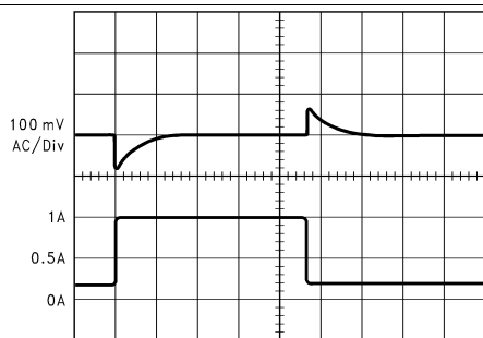
Figure 15. Continuous Mode Switching Waveforms, Horizontal Time Base: 1 \mu\text{s}/\text{div}
