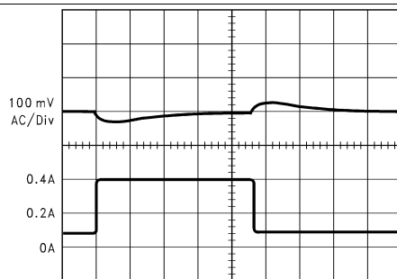
Figure 16. Discontinuous Mode Switching Waveforms, Horizontal Time Base: 1 \mu\text{s}/\text{div}
