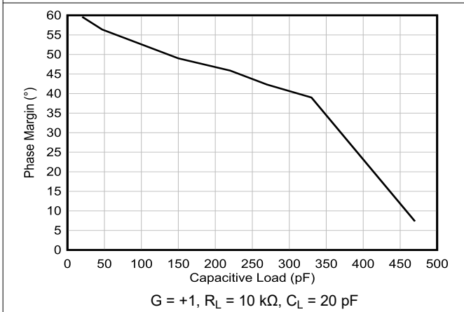
Figure 6-21. Phase Margin vs Capacitive Load
