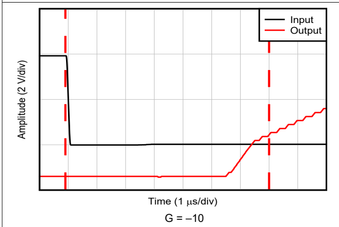
Figure 6-23. Overload Recovery (Negative Rail)
