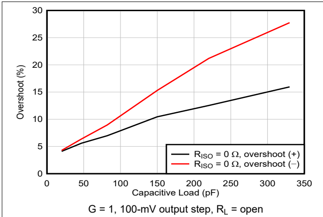
Figure 6-19. Small-Signal Overshoot vs Capacitive Load
