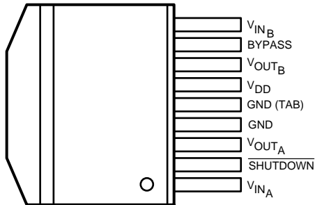
Figure 2. Plastic Package, DDPAK Top View See Package Number KTW0009A
