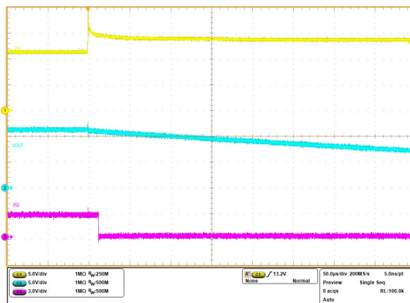
Figure 8-5. Overvoltage protection
