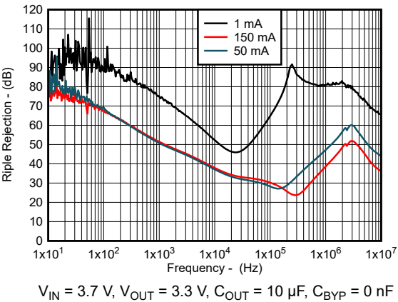
V_{IN} = 3.7\text{ V} , V_{OUT} = 3.3\text{ V} , C_{OUT} = 10\text{ }\mu\text{F} , C_{BYP} = 0\text{ nF} Figure 6-21. Ripple Rejection vs Frequency for New Chip
