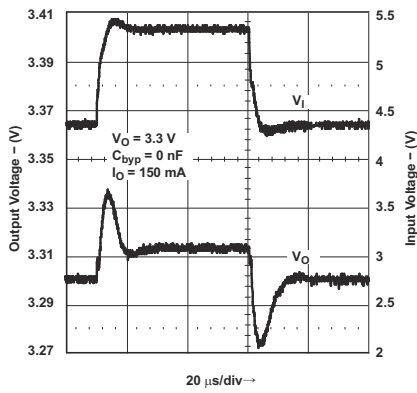
Figure 8-9. Line Transient Response for Legacy Chip
