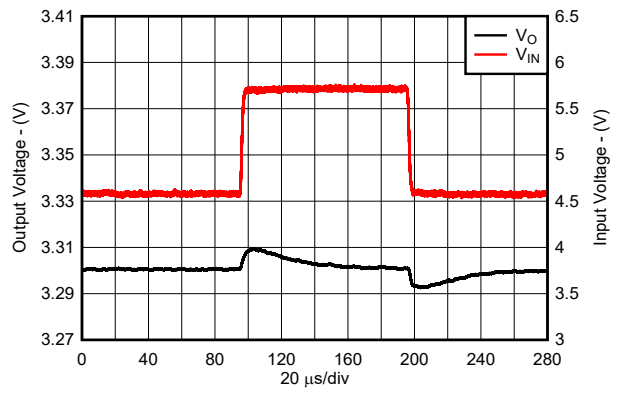
Figure 8-10. Line Transient Response for New Chip
