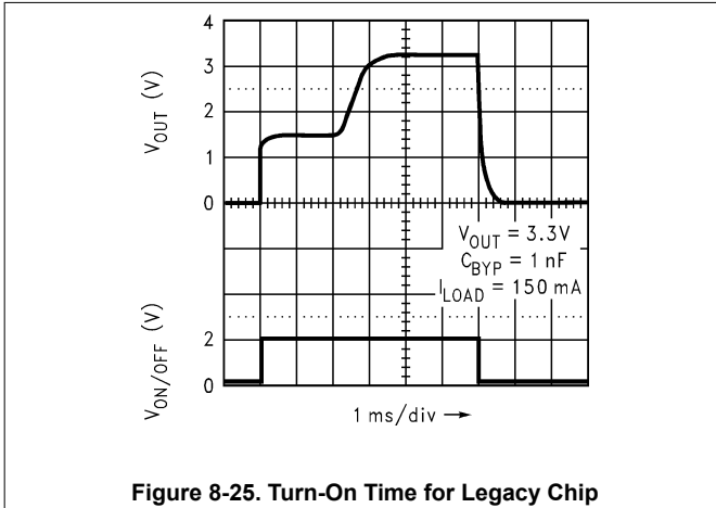
Figure 8-25. Turn-On Time for Legacy Chip
