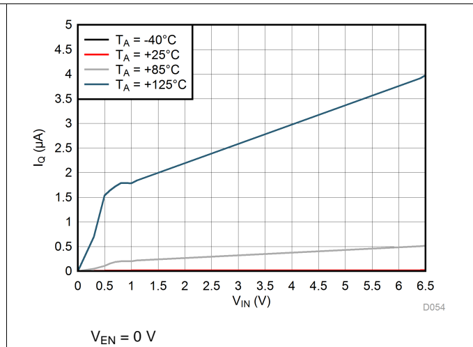
Figure 14. LP5912-0.9 I_{Q(SD)} vs V_{IN}
