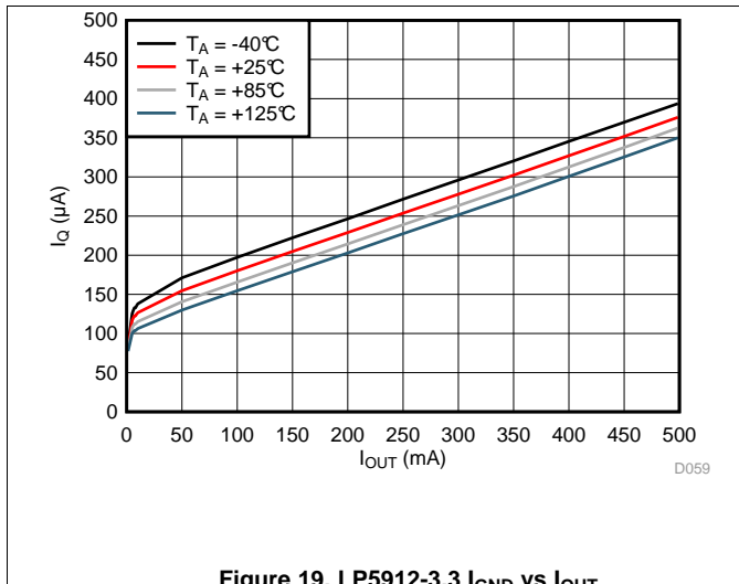
Figure 19. LP5912-3.3 I_{GND} vs I_{OUT}
