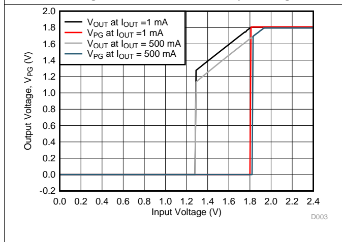
Figure 3. LP5912-1.8 Output Voltage, V_{PG} vs Input Voltage
