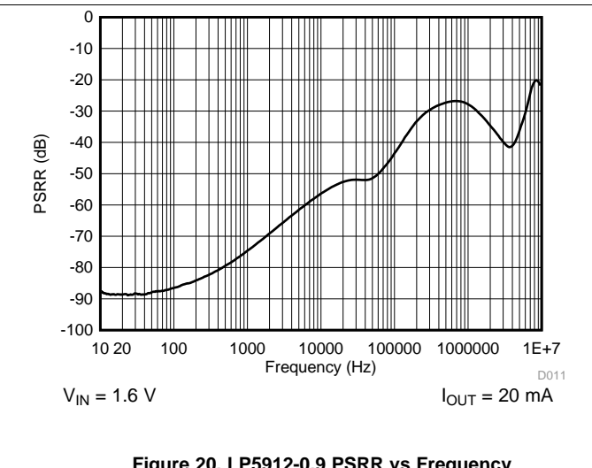
Figure 20. LP5912-0.9 PSRR vs Frequency
