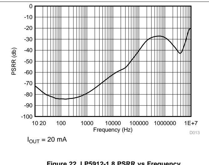
Figure 22. LP5912-1.8 PSRR vs Frequency
