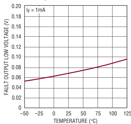
Fault Output Low Voltage vs Temperature
