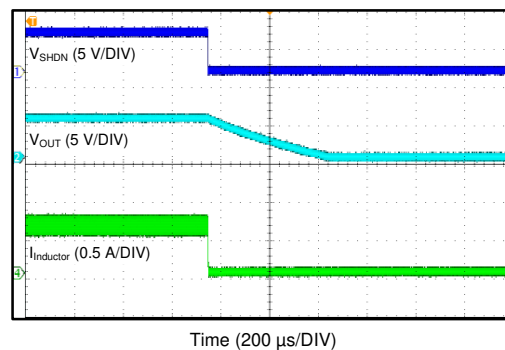
Figure 8-7. Shutdown Waveform
