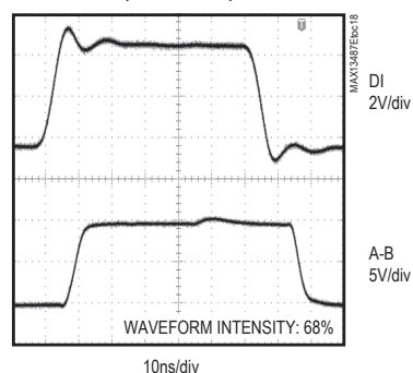
DRIVER PROPAGATION (16Mbps) (MAX13488E)
