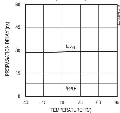
RECEIVER PROPAGATION vs. TEMPERATURE (MAX13487E)
