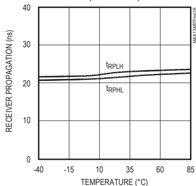
RECEIVER PROPAGATION vs. TEMPERATURE (MAX13488E)
