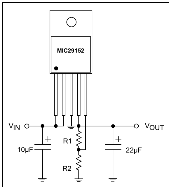
FIGURE 4-2: Adjustable Regulator with Resistors.
