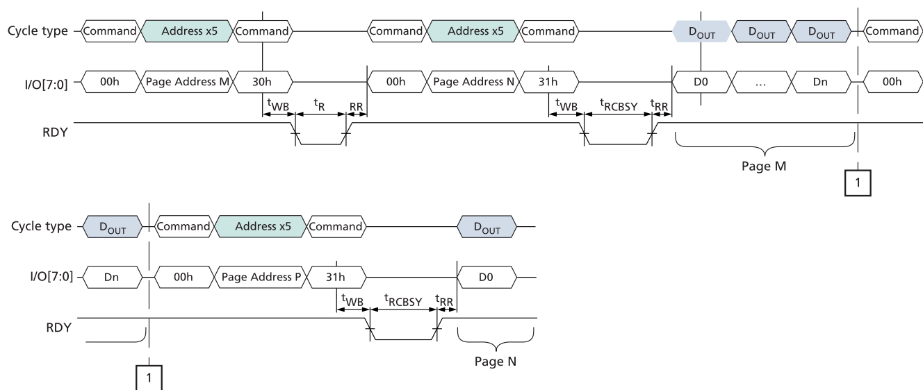
Figure 41: READ PAGE CACHE RANDOM (00h-31h) Operation
