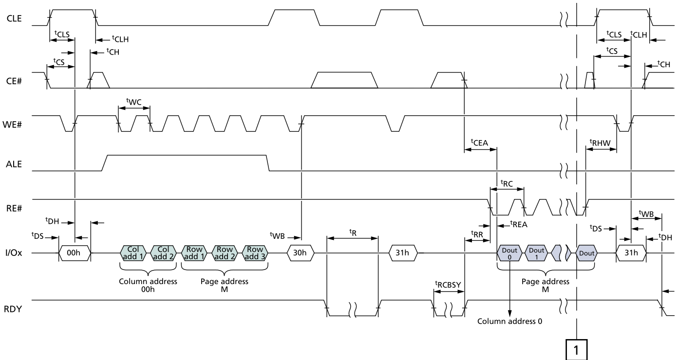
Figure 89: READ PAGE CACHE SEQUENTIAL
