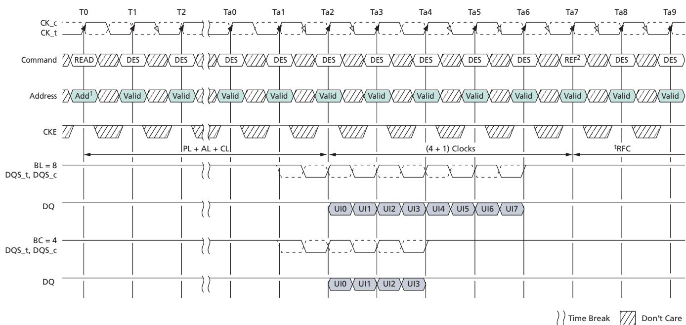
Figure 41: READ-to-REFRESH Timing
