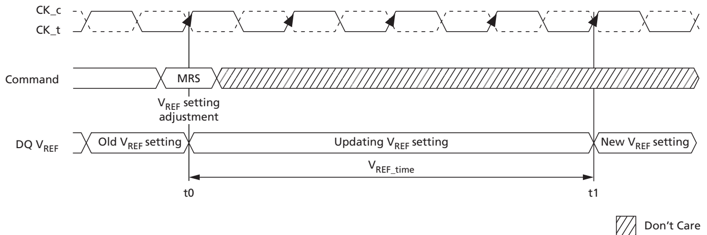
Figure 66: V_{\text{REFDQ}} Timing Diagram for V_{\text{REF,time}} Parameter
