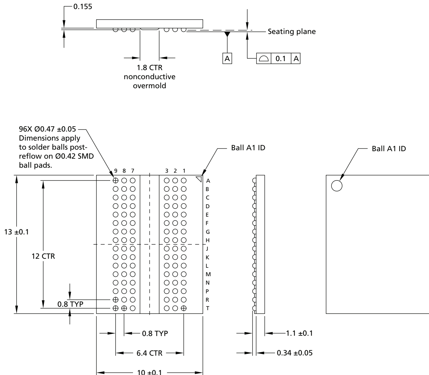
Figure 10: 96-Ball FBGA – x16 (RC)
