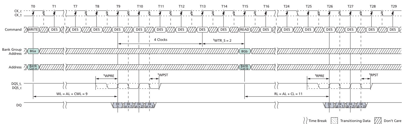
Figure 185: WRITE (BC4) OTF to READ (BC4) OTF with 1^{\text{t}}\text{CK} Preamble in Different Bank Group
