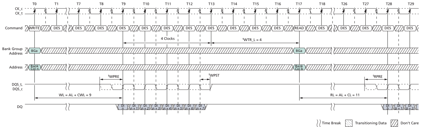
Figure 184: WRITE (BL8) to READ (BL8) with 1^{\text{t}}\text{CK} Preamble in Same Bank Group
