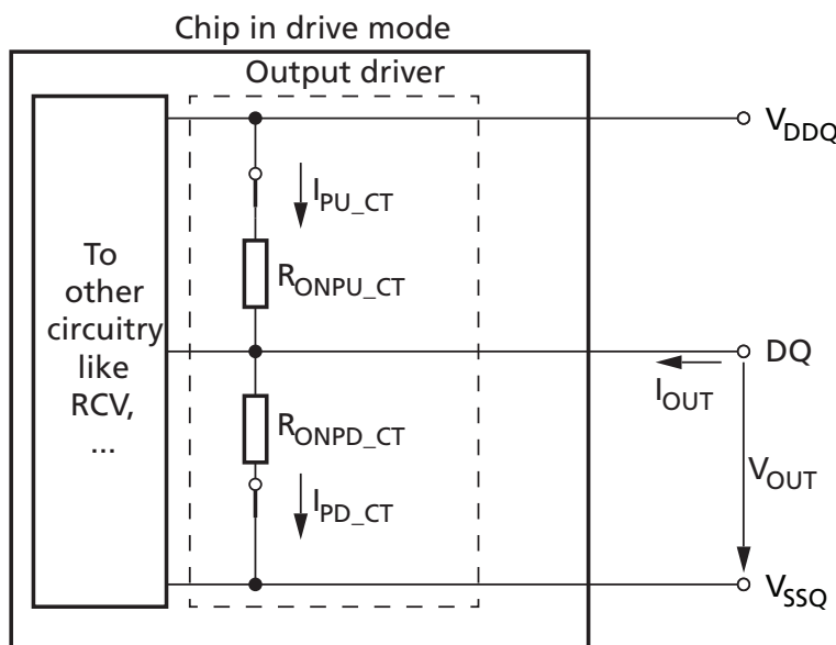
Figure 236: Output Driver During Connectivity Test Mode
