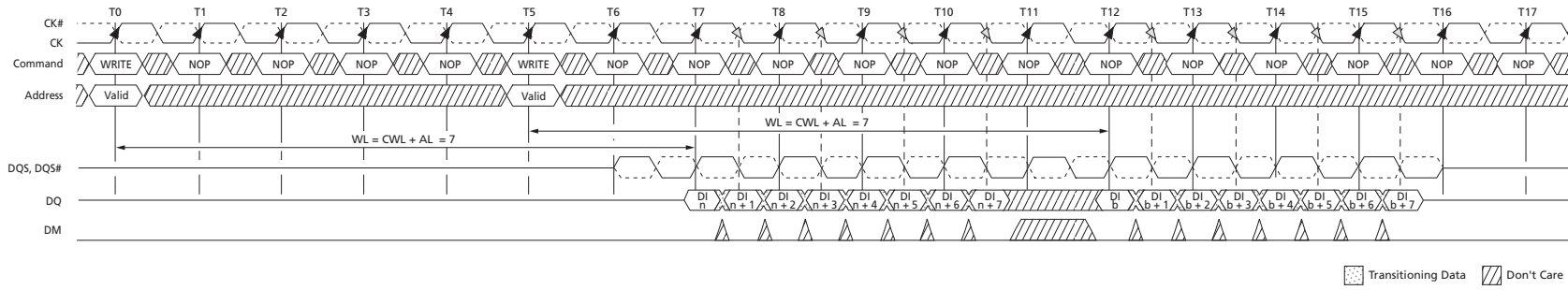
Figure 87: Nonconsecutive WRITE to WRITE
