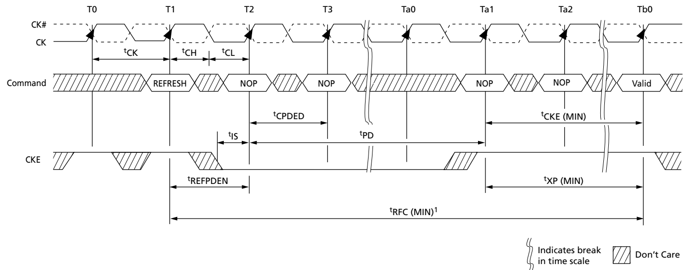
Figure 100: REFRESH to Power-Down Entry
