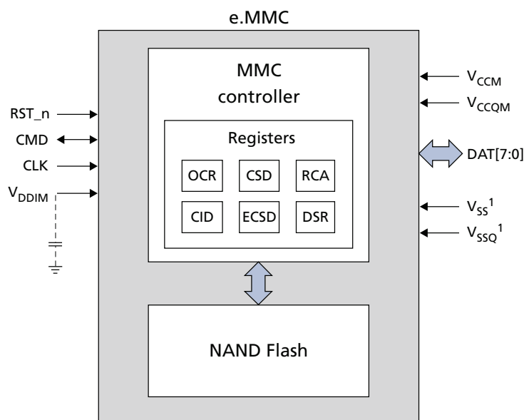
Figure 5: e.MMC Functional Block Diagram
