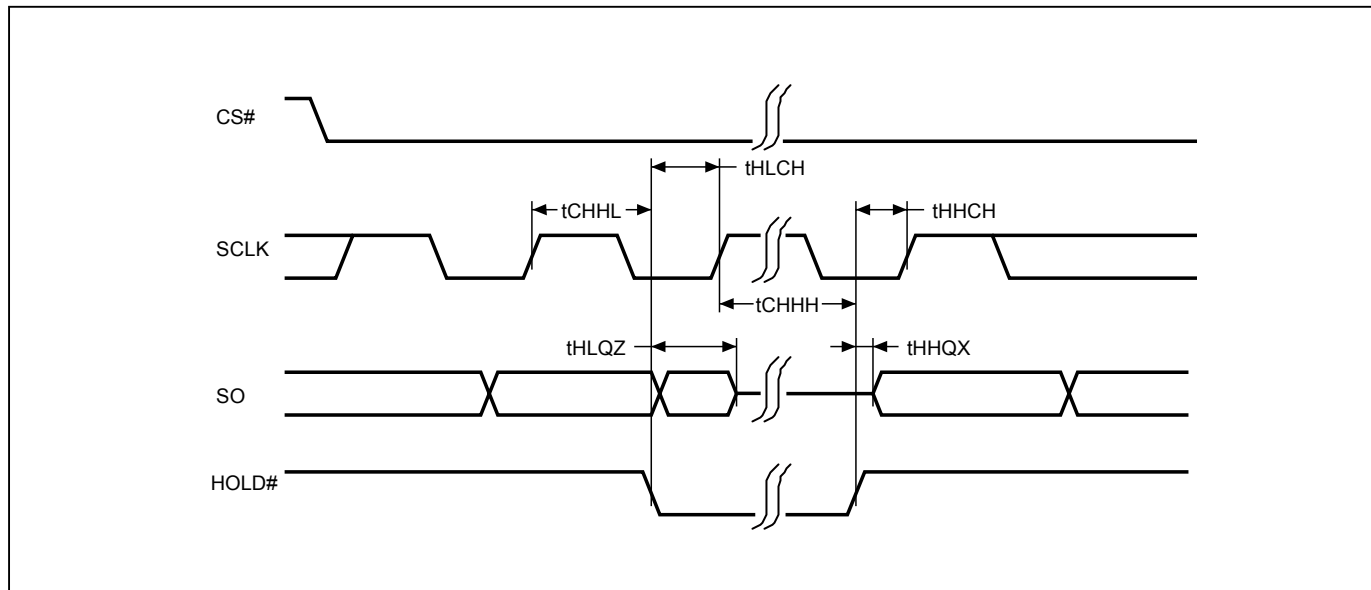
Figure 11. Hold Timing
