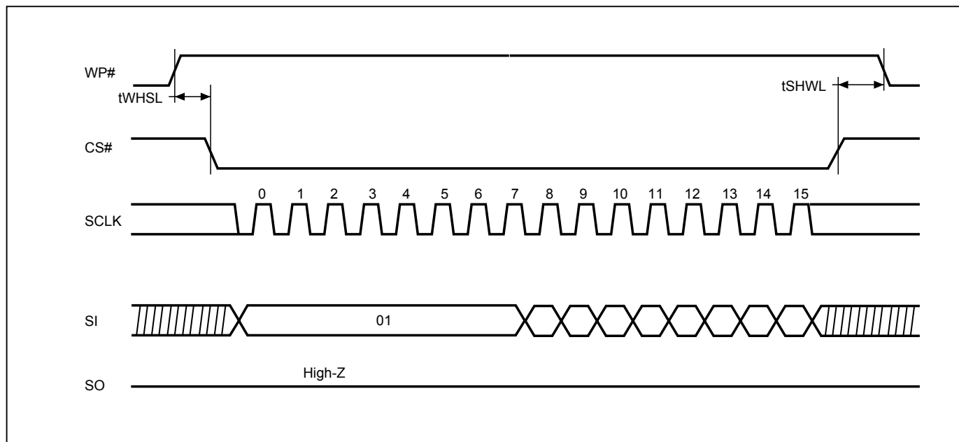
Figure 12. WP# Disable Setup and Hold Timing during WRSR when SRWD=1
