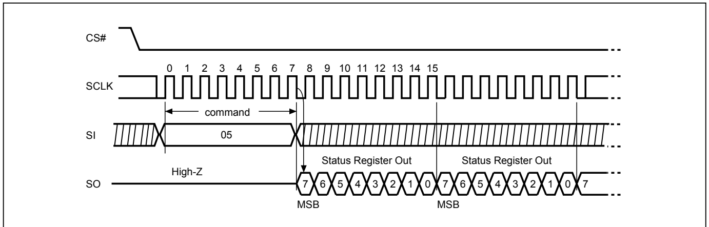
Figure 15. Read Status Register (RDSR) Sequence (Command 05h)
