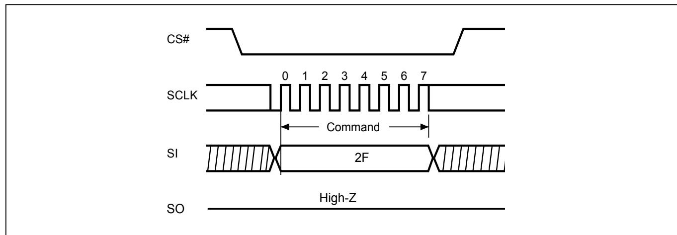
Figure 30. Write Security Register (WRSCUR) Sequence (Command 2Fh)
