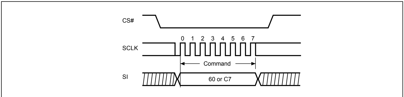
Figure 22. Chip Erase (CE) Sequence (Command 60h or C7h)
