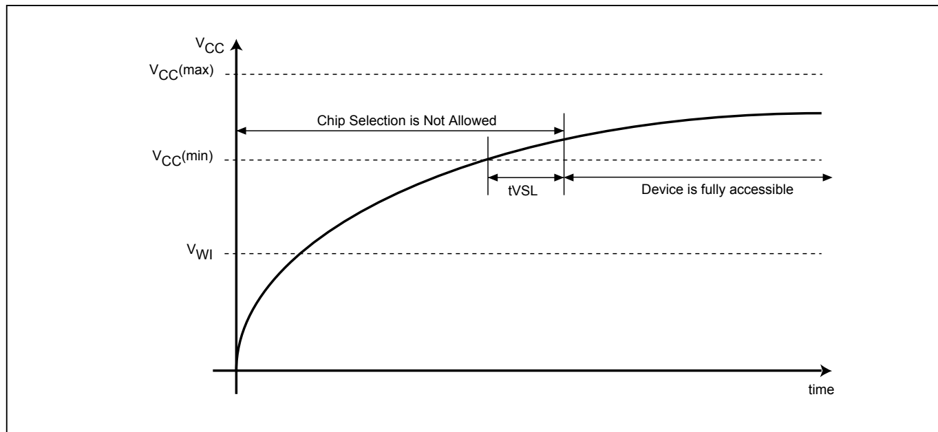
Figure 99. Power-up Timing
