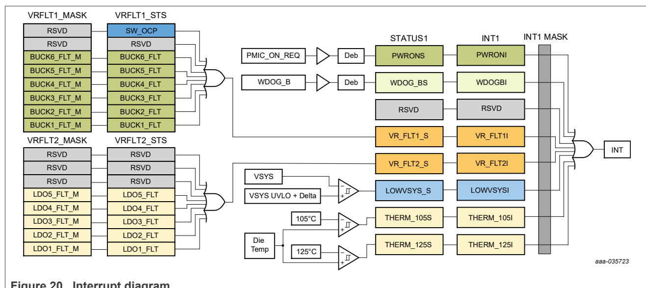
Figure 20. Interrupt diagram
