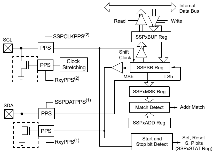
FIGURE 32-3: MSSP BLOCK DIAGRAM (I 2 C CLIENT MODE)
