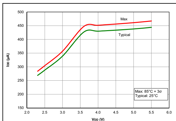
FIGURE 36-2: I_{DD} , XT Oscillator, 4 MHz, PIC16F18324/18344 Only
