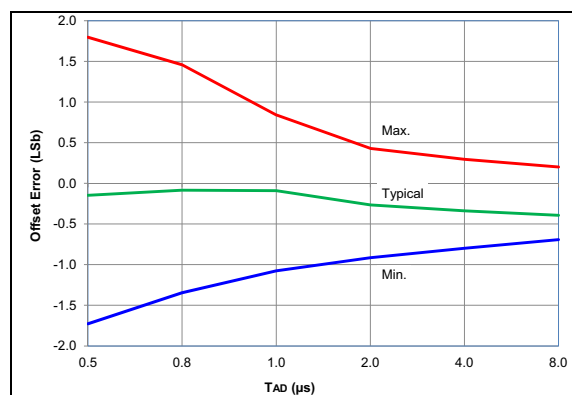
FIGURE 36-66: ADC 10-Bit Mode, Single-Ended Offset Error, V_{DD} = 3.0V , V_{REF} = 3.0V , -40^{\circ}C to 85^{\circ}C , All devices
